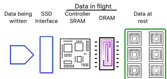
Figure 8: PLP Client SSD with DRAM
